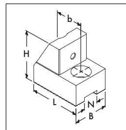
Trägerbacke TRQ...-2 Support Jaw TRQ...-2
